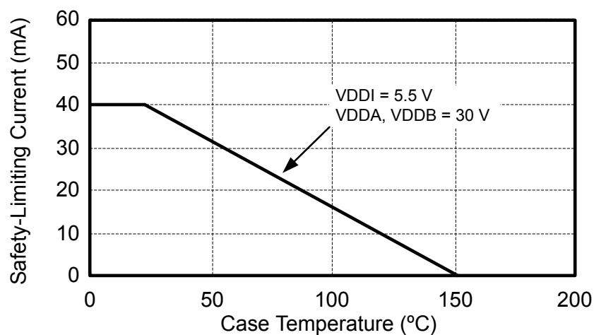
Figure 4.4. NB SOIC-16, LGA-14 Thermal Derating Curve, Dependence of Safety Limiting Values Limiting Values with Case Temperature per VDE 0884
