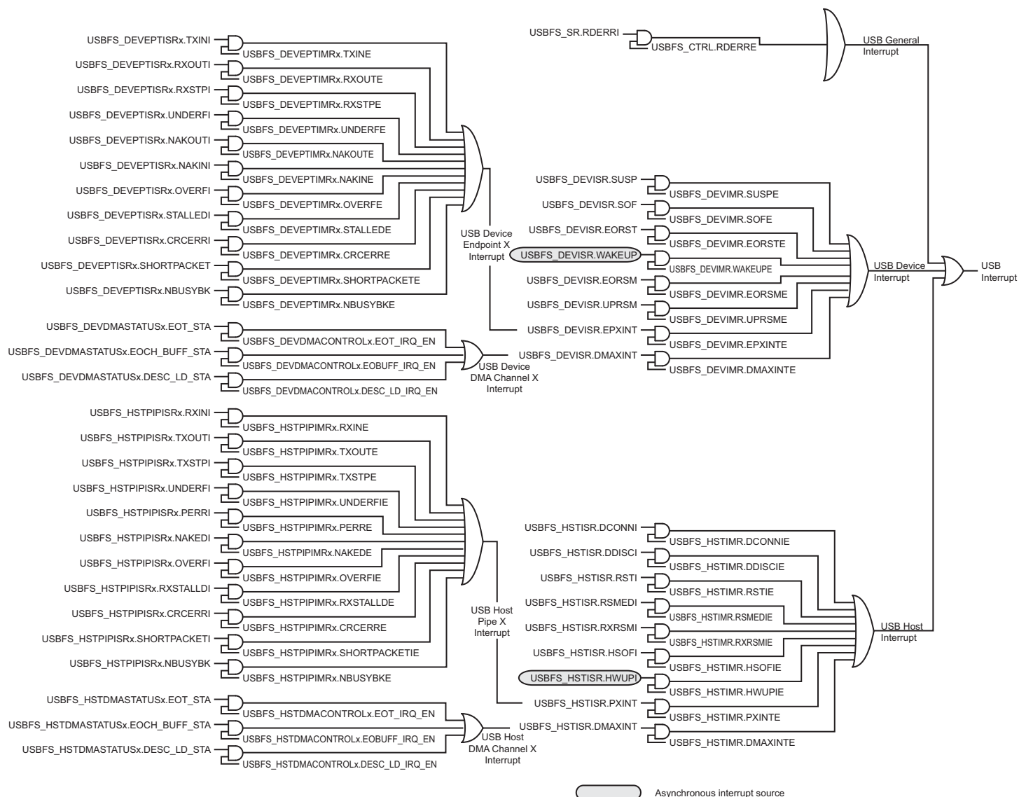
Figure 45-6. Interrupt System
