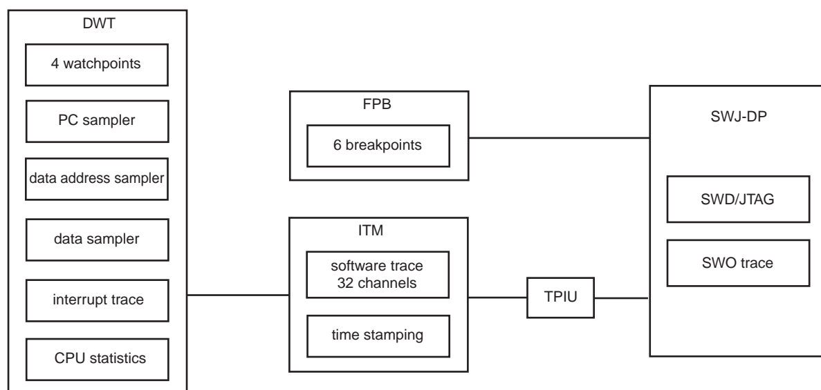
Figure 13-5. Debug Architecture
