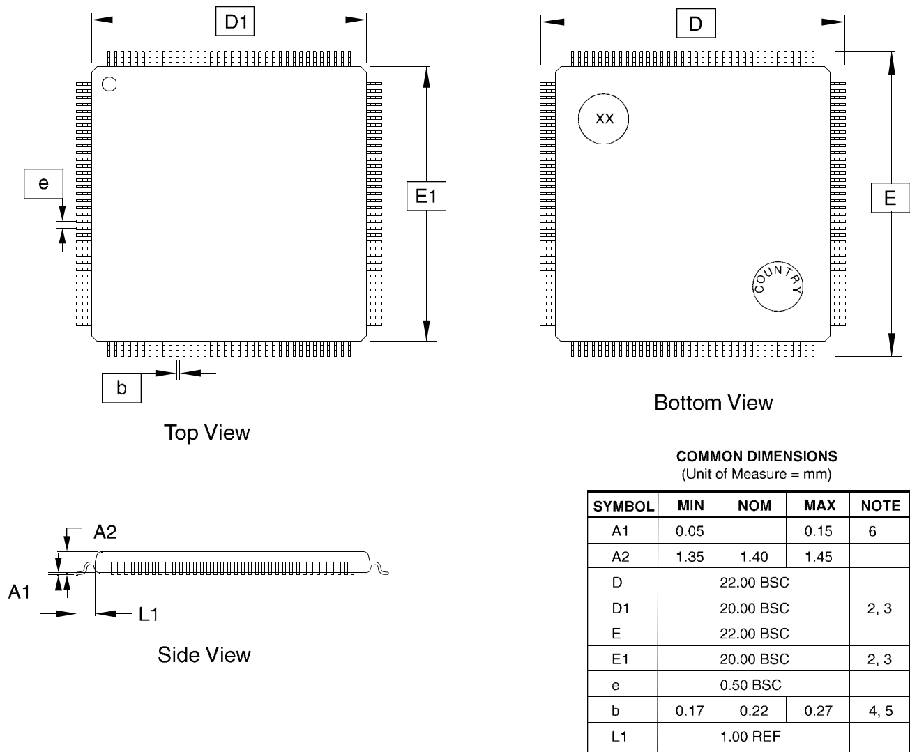
Figure 47-2. 144-lead LQFP Package Mechanical Drawing
