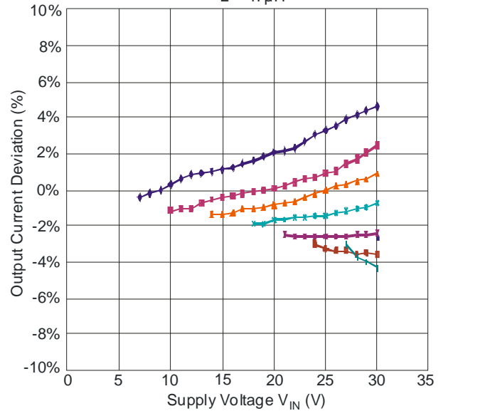
ZXLD1360 Output Current L = 47\mu\text{H}
