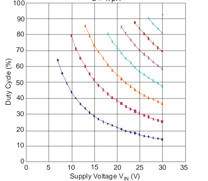
ZXLD1360 Duty Cycle L = 47\mu\text{H}
