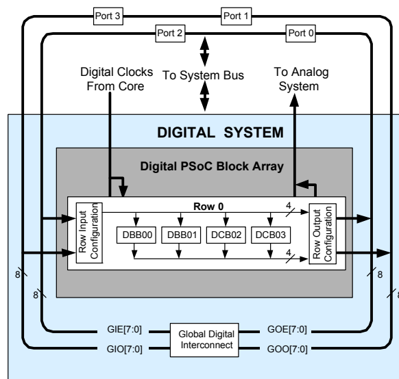
Figure 1. Digital System Block Diagram
