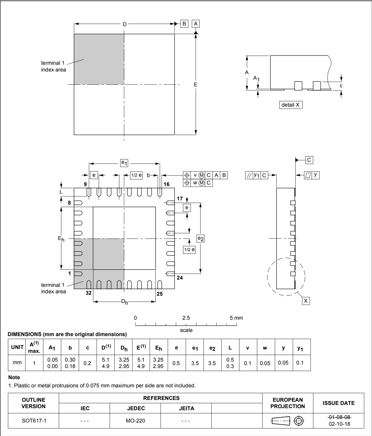
Figure 37. Package outline SOT-617-1 (HVQFN32)
