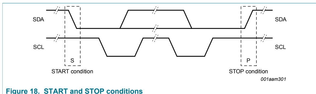
Figure 18. START and STOP conditions
