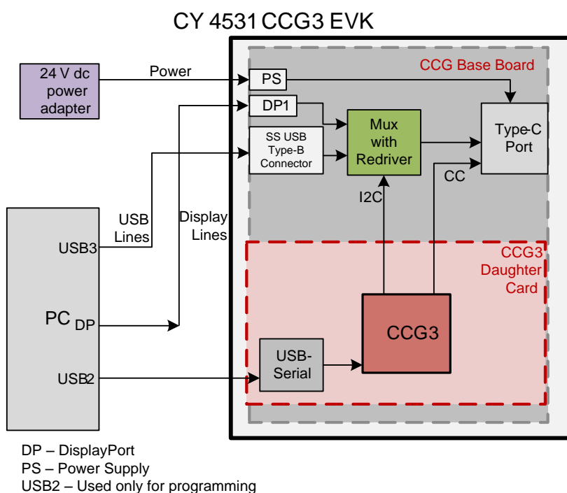
Figure 3-1: CY4531 EZ-PD CCG3 EVK Architecture
