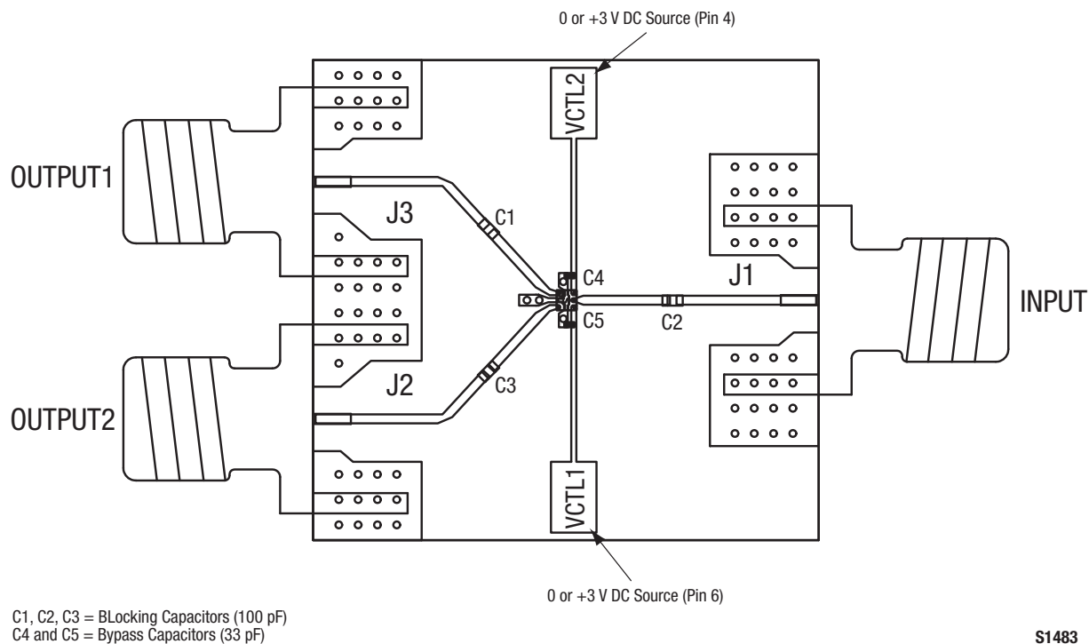
Figure 9. SKY1323-378LF Evaluation Board Assembly Diagram
