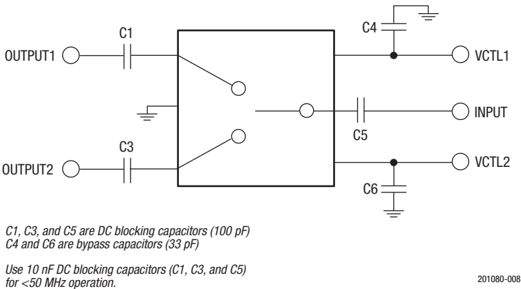
Figure 8. SKY13323-378LF Evaluation Board Schematic
