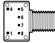
BOTTOM VIEW, HFBR-2505AFZ/BFZ
