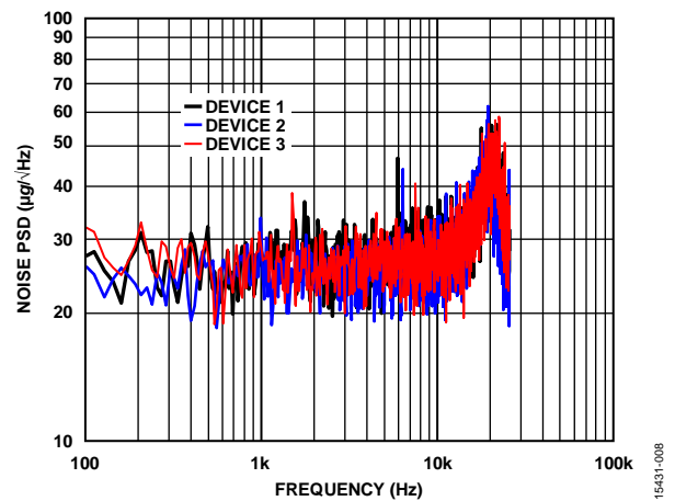
Figure 8. ADXL1002 Noise Power Spectral Density (PSD) vs. Frequency
