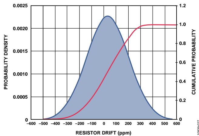
Figure 28. Resistor Lifetime Drift
