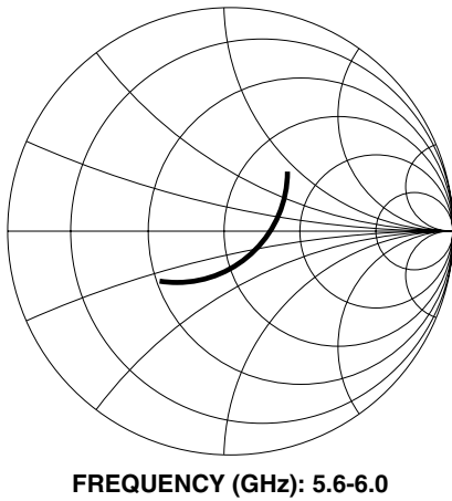
Figure 22. Input Impedance.
